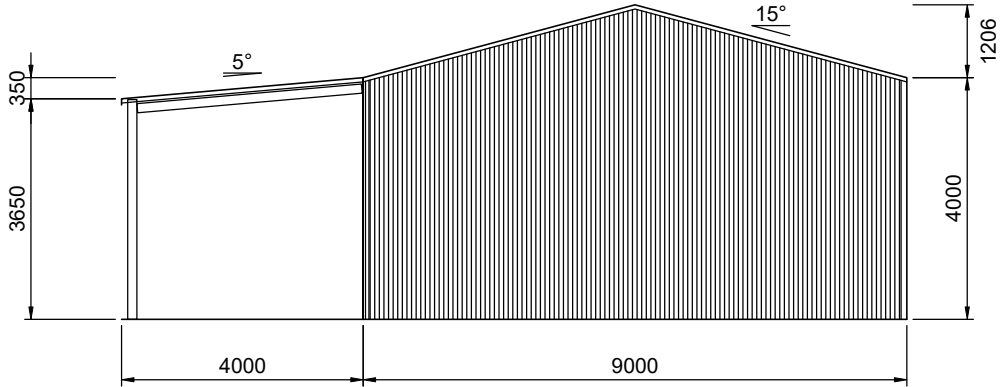
3 2 REAR BUILDING ELEVATION SCALE: 1:125
