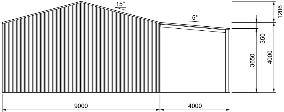
4 2 FRONT BUILDING ELEVATION SCALE: 1:125
