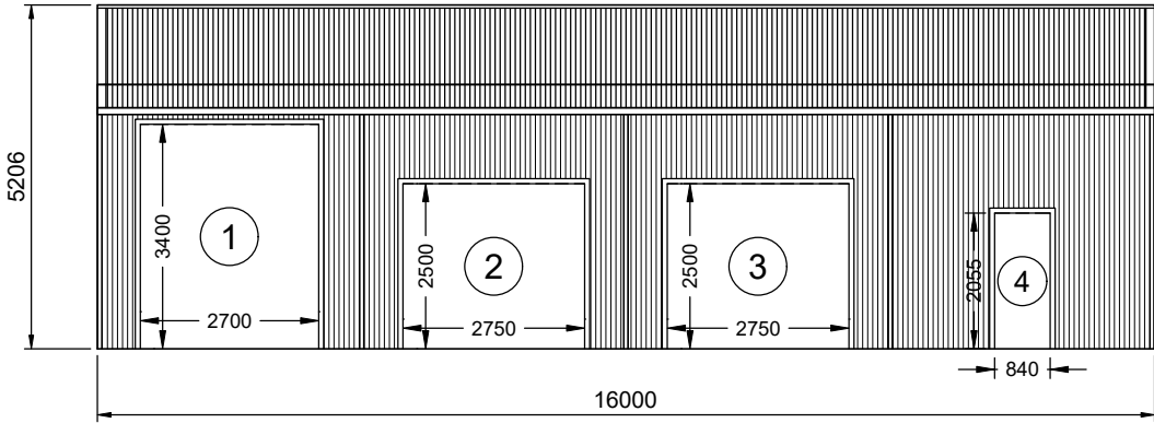
1 2 SIDEWALL A BUILDING ELEVATION SCALE: 1:125
